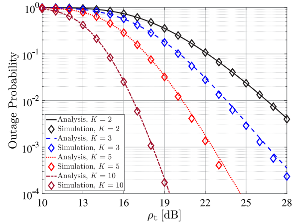
Fig. 2. OP performance of C-STLC according to \rho_t with various K .
