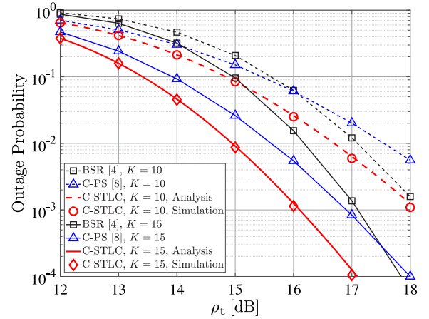
Fig. 3. OP performance of C-STLC, BSR, and C-PS according to \rho_t .
