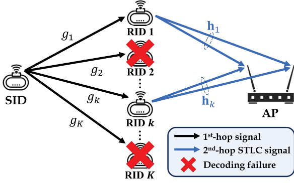
Fig. 1. System model of the proposed C-STLC for R-IoT.
